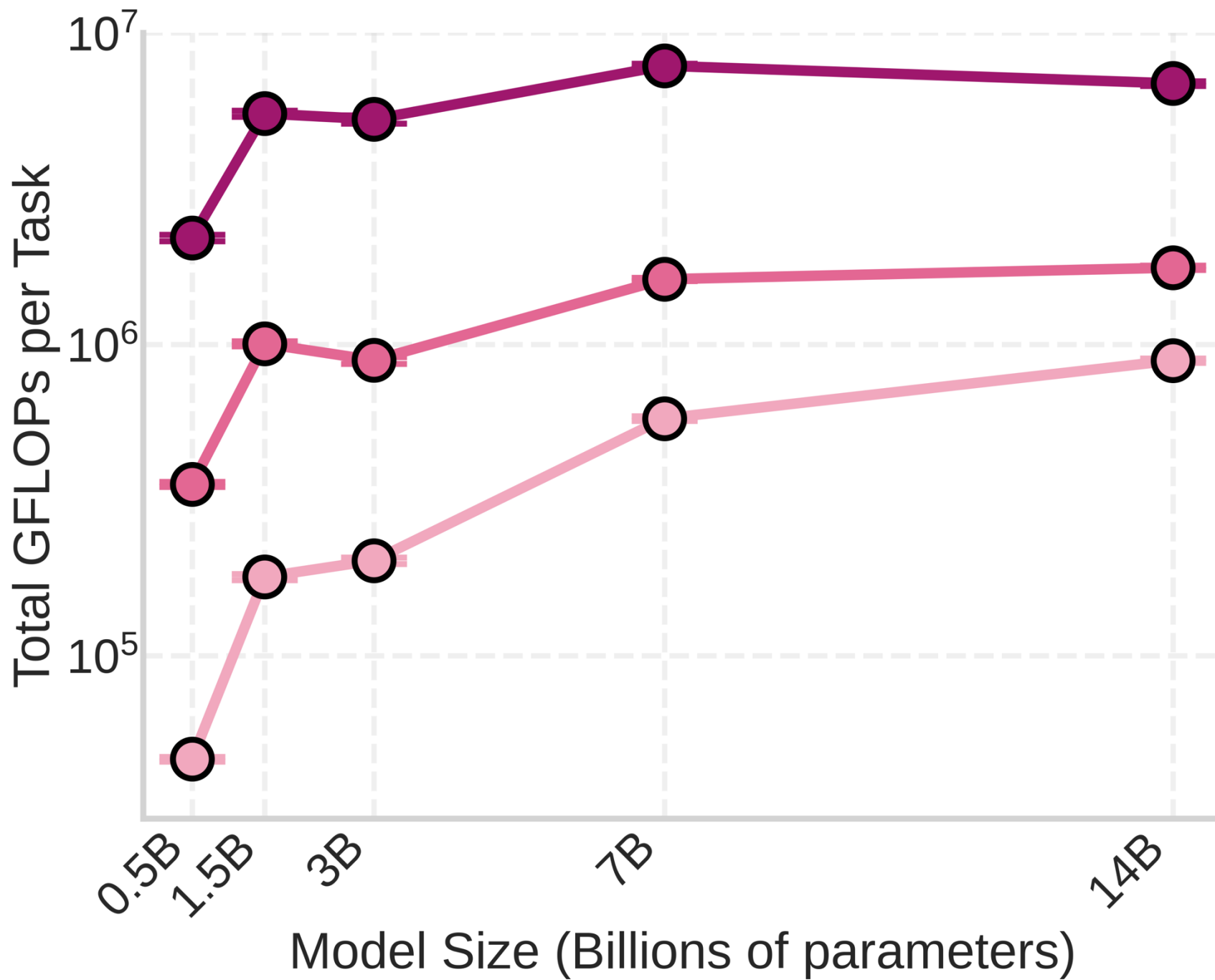
Total FLOPs versus Compressor Size
