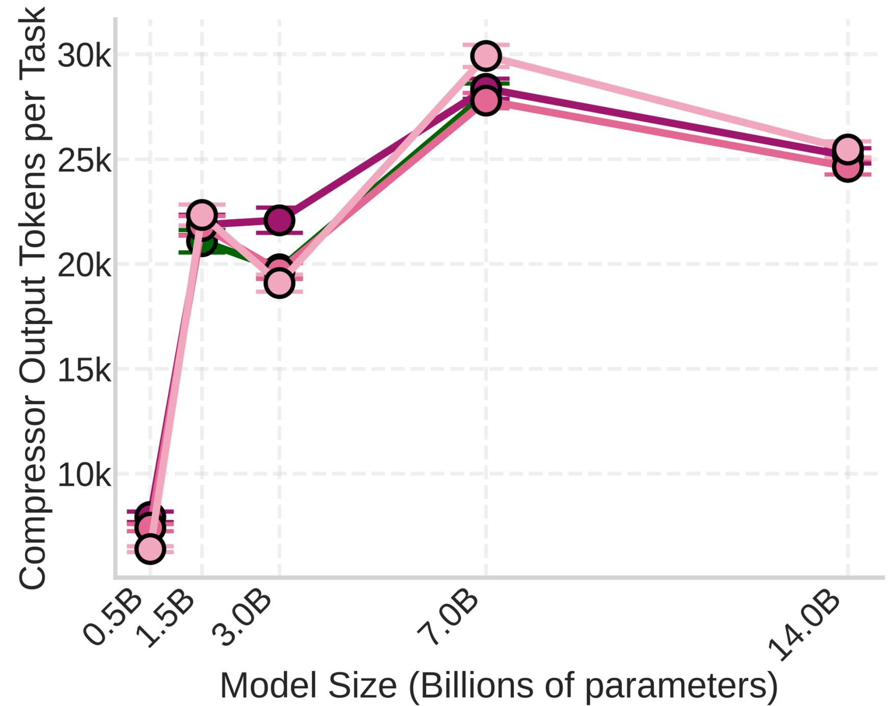
Compressor Output Tokens versus Compressor Size
